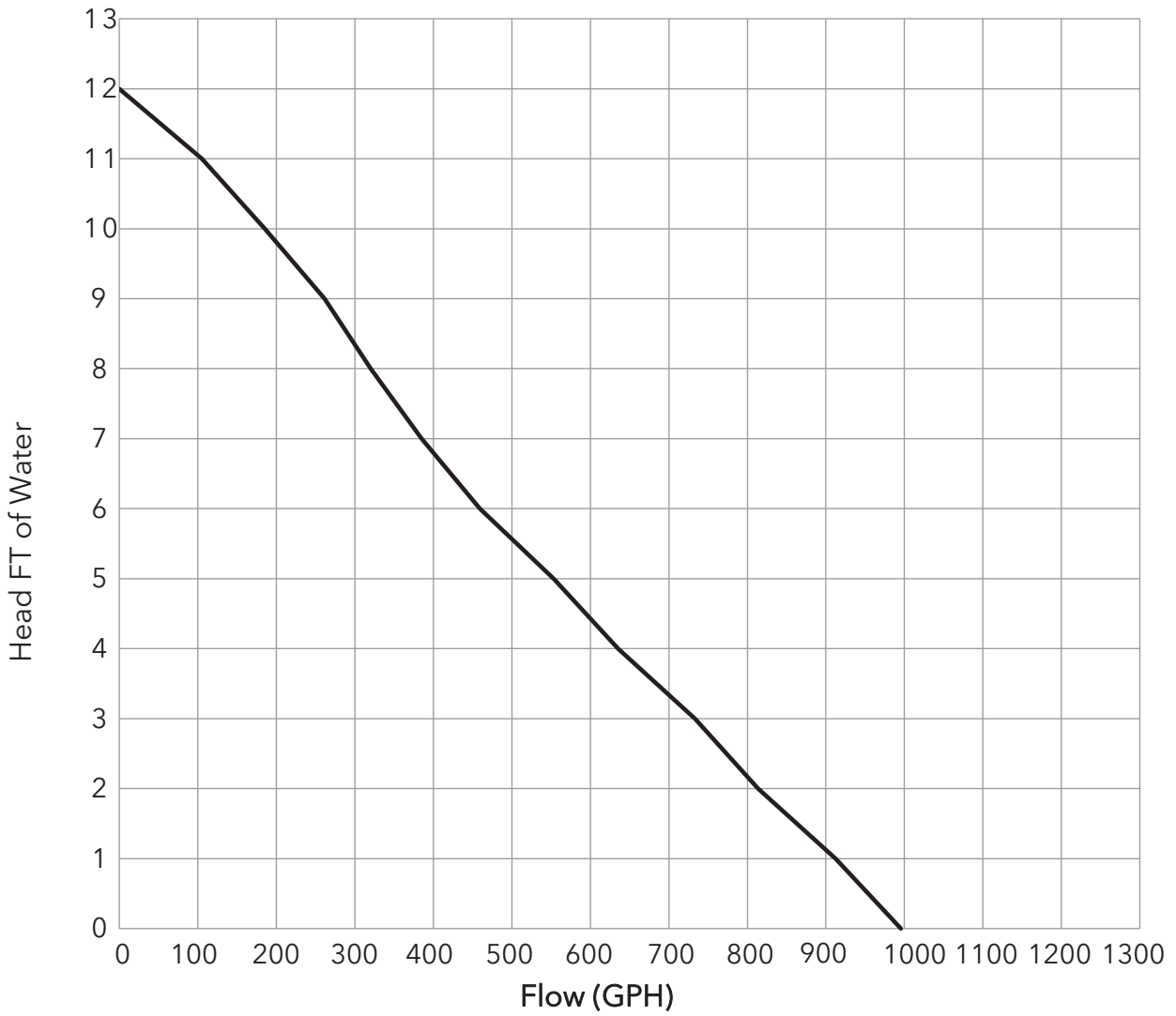
800 GPH Bilge Pump Performance at 12 Volts
