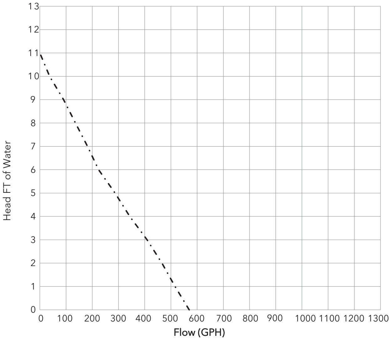
500 GPH Bilge Pump Performance at 12 Volts
