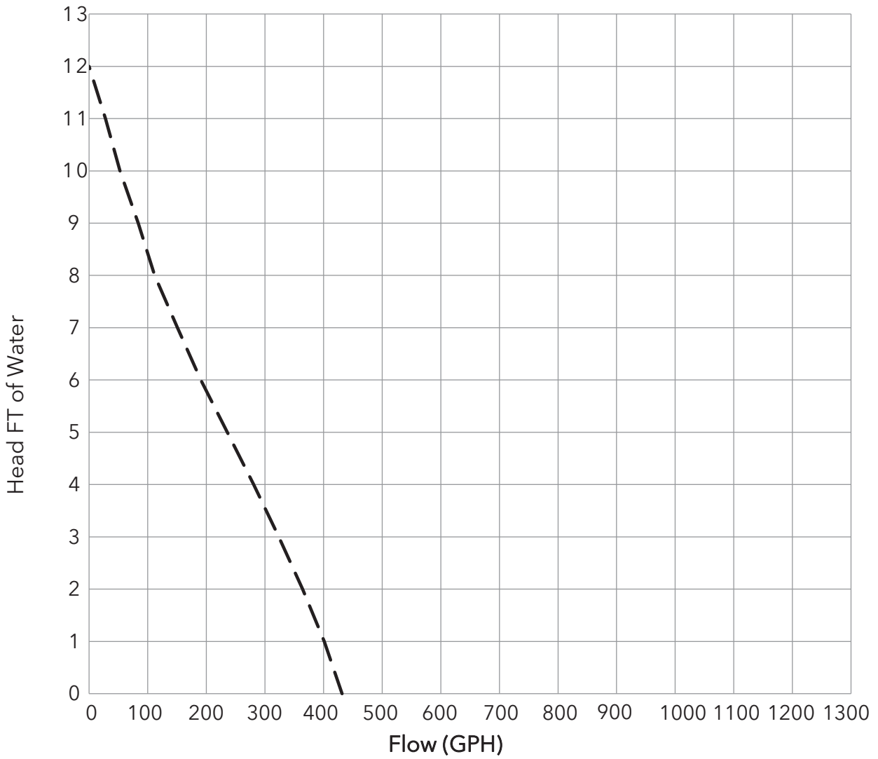
360 GPH Bilge Pump Performance at 12 Volts
