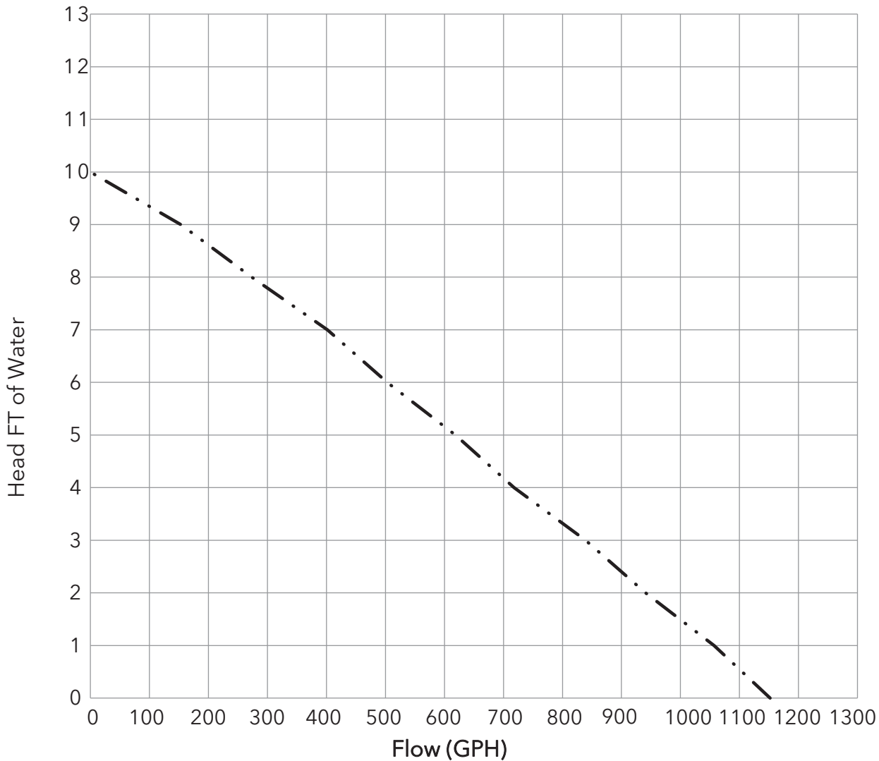
1100 GPH Bilge Pump Performance at 12 Volts
