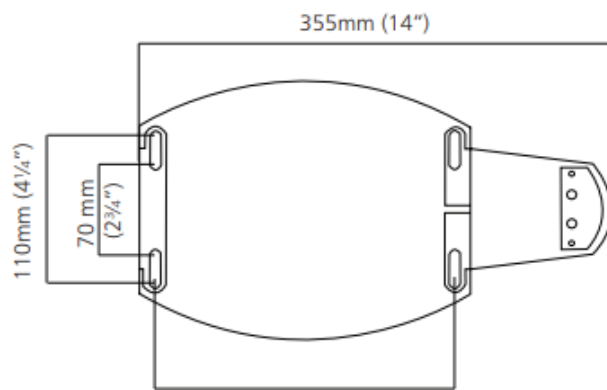
Lite Flush Footprint
