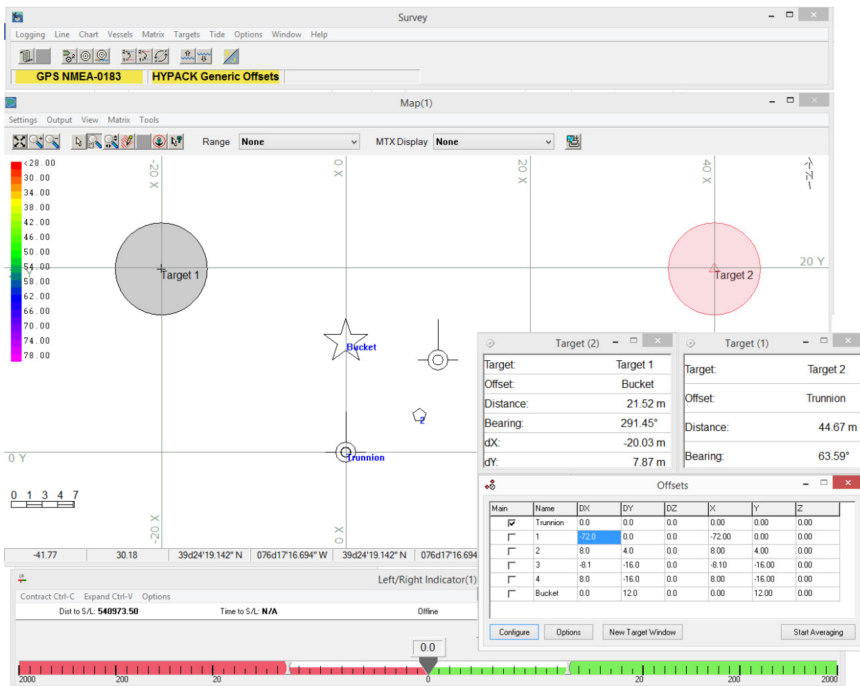
FIGURE 4. SURVEY Program Running with a Couple of Offset to Target Windows
