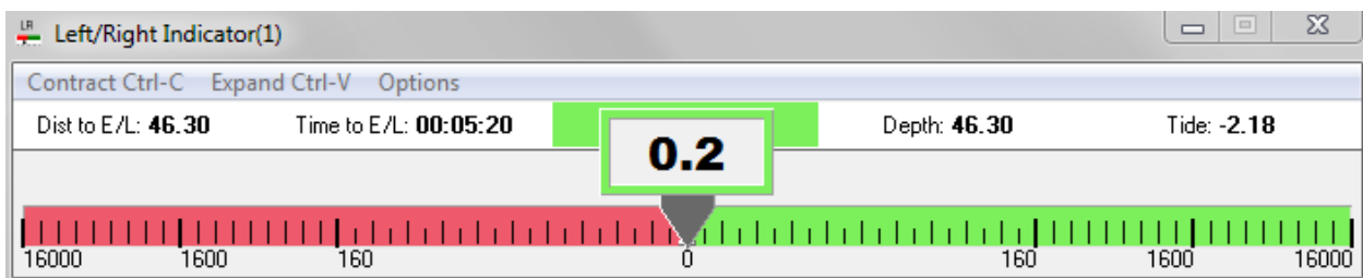
FIGURE 3. New L/R Indicator showing Distance/Time to End of Line - "Dist. to E/L" and "Time to E/L"
