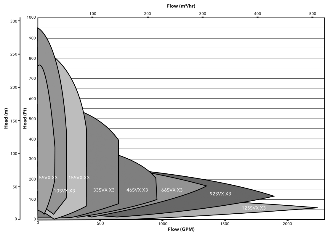
e-HVX Family Curve
