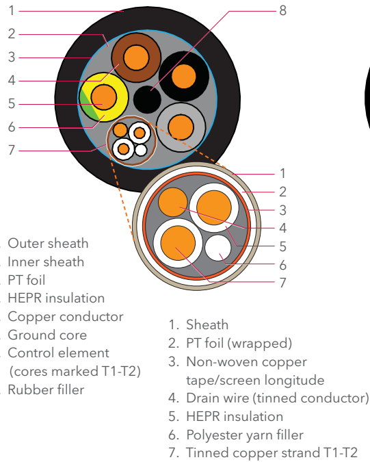
4G10+S(2x0.5) SUBCAB®
