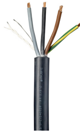
4G10+S(2x0.5) SUBCAB®
