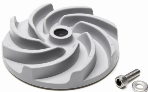
Impeller kit including torque flow impeller, plain washer, hexagon socket head screw and a mounting instruction.
