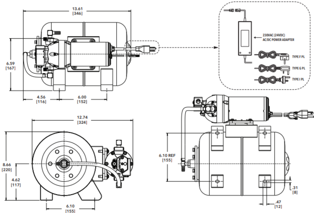
2 gallon (7.57 liter) models Inches [millimeters]
