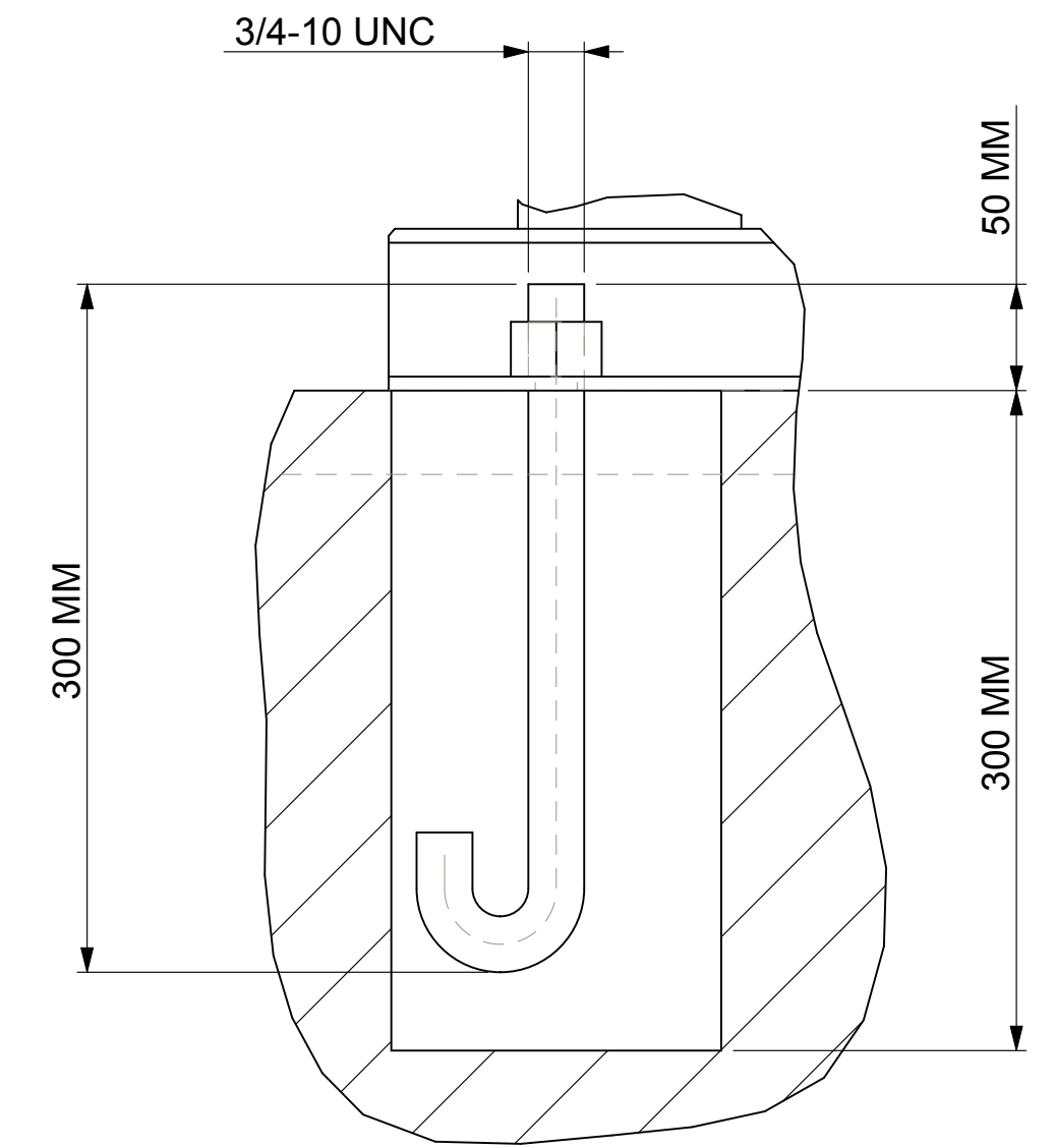
DETAIL A SCALE 0.286
