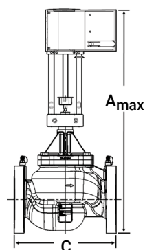
Model PVL 2-1/2" – 6"
