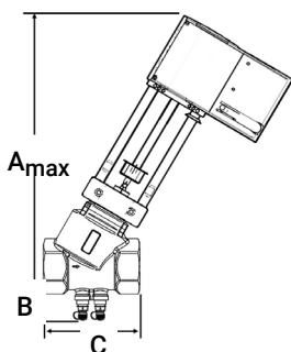
Model PVC 1-1/2" – 2"
