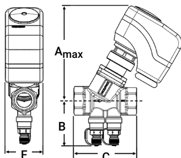
Model PVC 1/2" – 1-1/4"
