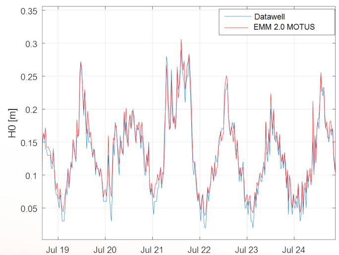
Figure 16: Significant wave height from the EMM2.0 MOTUS Buoy and the Waverider in the Bjørnafjorden.
