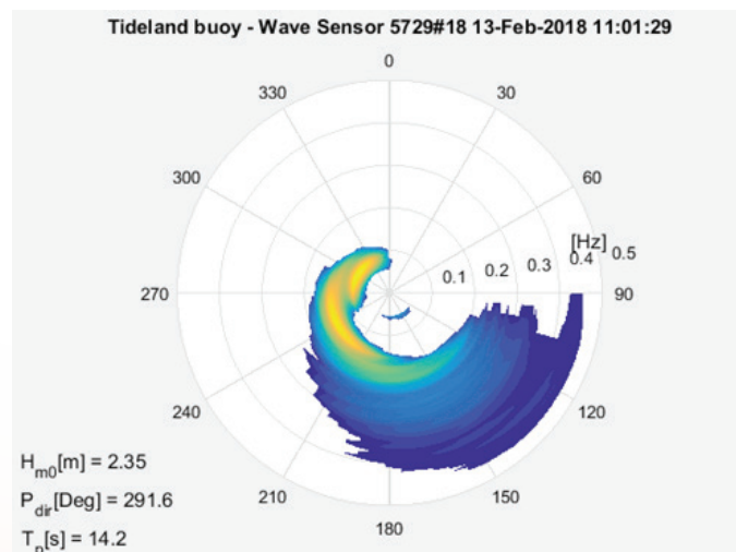
Figure 13: Example of the representation of the directional energy spectrum revealing two dominant wave fields, separated by frequency and direction.
