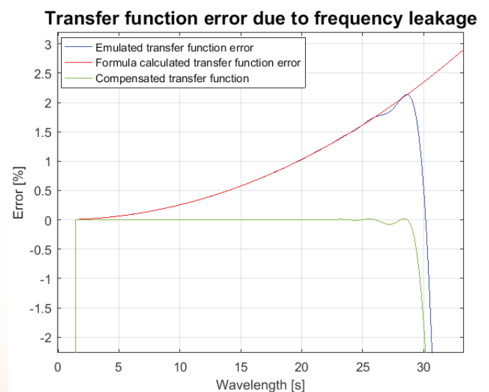
Figure 4: Transfer function error due to frequency leakage
