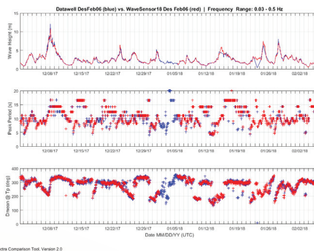
Figure 8: CDIP WaveEvalTool time domain comparison. Comparison of wave height (upper graph), peak period (graph in the middle) and peak direction (lower graph) shows excellent agreement between the Waverider and the three MOTUS Sensors on two buoys (Navigational and Environmental). This example represents the comparison between Datawell and the MOTUS Sensor number 18 in the Tideland Buoy.
