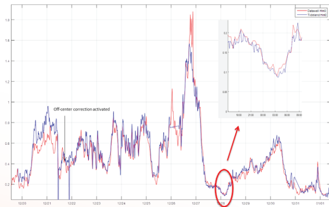
Figure 15: Significant wave height from Datawell waverider and Tideland MOTUS Buoy deployed in the Bjørnafjorden.
