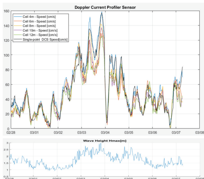
Figure 12: Eddy observation: The first graph represents the current values from the surface down to 12m. The second graph represents the wave height during the same period. Before the 4th of March 2018, currents have increased gradually and then decreased rapidly down to few centimeters.
