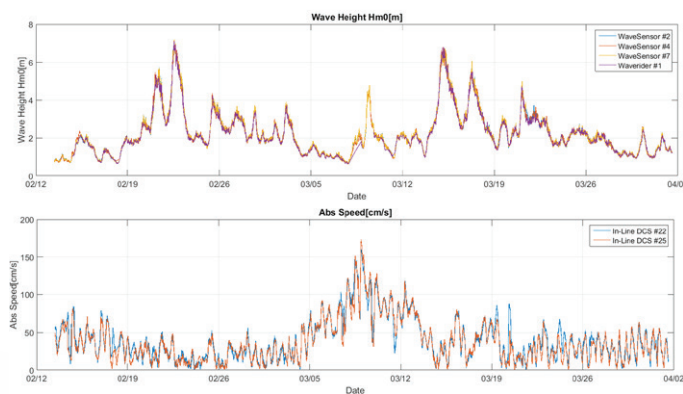
Figure 10: Wave height from four sensors (upper graph) and surface currents from the two Xylem buoys from the 12th of February to the 2nd of April. Around the 8th of March, an event with currents over 150 cm/s and 4m significant wave height was registered. During this event, the data transmission from the Waverider buoy is lost during a period of time due to the buoy submersion while the MOTUS Buoys provide good and reliable data.
