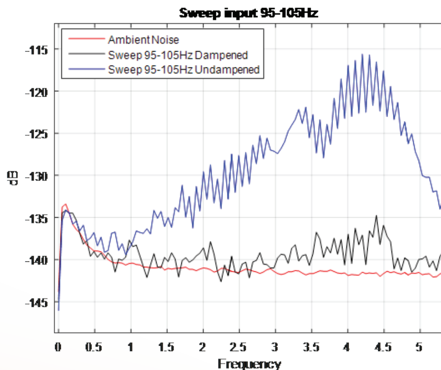
Figure 2: Effect of the mechanical filter. The blue curve represents the noise induced by the shaker plate. The black curve represents the noise while using the mechanical filter and the red curve represents the ambient noise without any shaker plate excitation.
