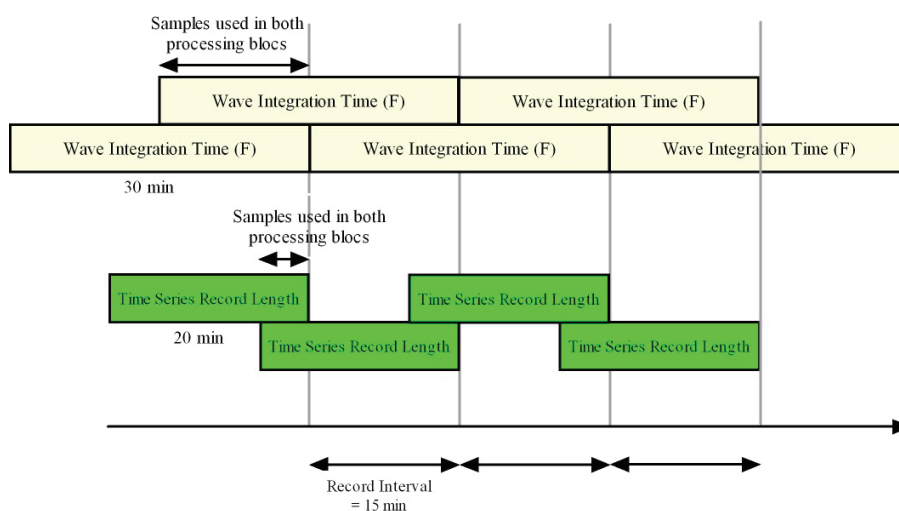
Figure 1: In this example, data are given out every 15 minutes as defined by the recording interval. The wave integration time sets the duration for the frequency domain based calculation, 30 minutes in this example. So every 15 minutes the parameters for the frequency domain will be calculated using the data samples from the 30 previous minutes.
