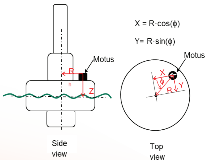
Figure 3: Illustration of off-center installation of MOTUS Sensor
